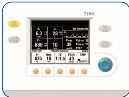
Optional pressure waveform provides a quick visual reference of the breath type and pressure level on the 7100 ventilator
